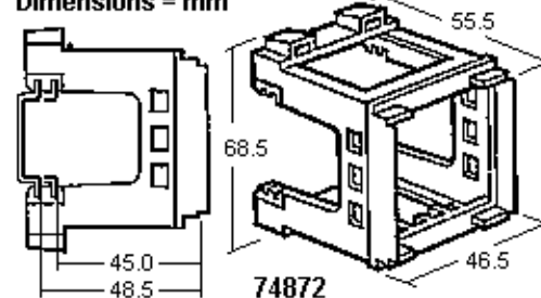
Dimensions = mm
