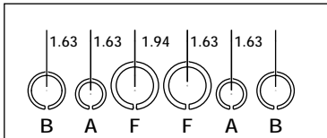
12" SIDE
